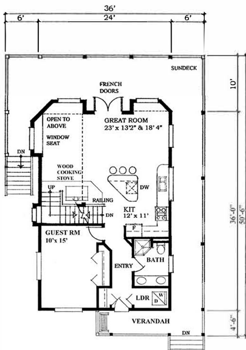
FIRST FLOOR PLAN AREA: 902 SQ. FT. TOTAL AREA: 1538 SQ. FT.
