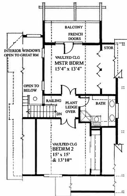
SECOND FLOOR PLAN AREA: 636 SQ. FT.
